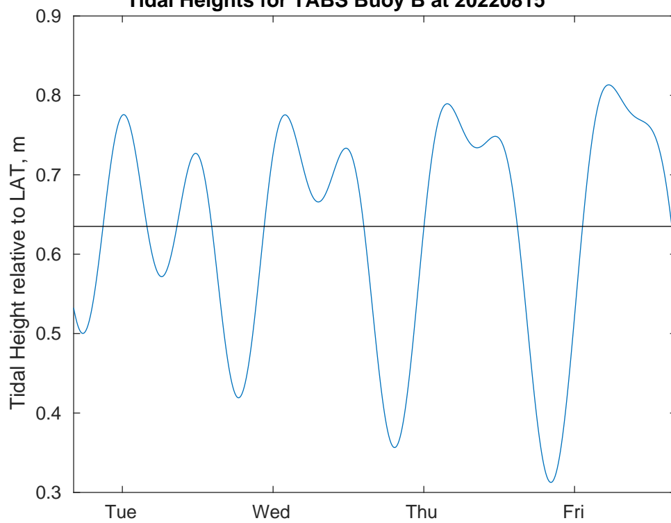
Tidal Heights for TABS Buoy B at 20220815
